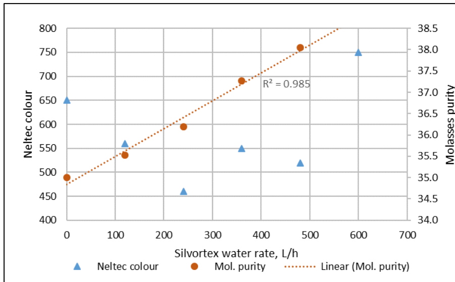
Figure 16 Effect of water distribution on Neltec colour and molasses purity.
