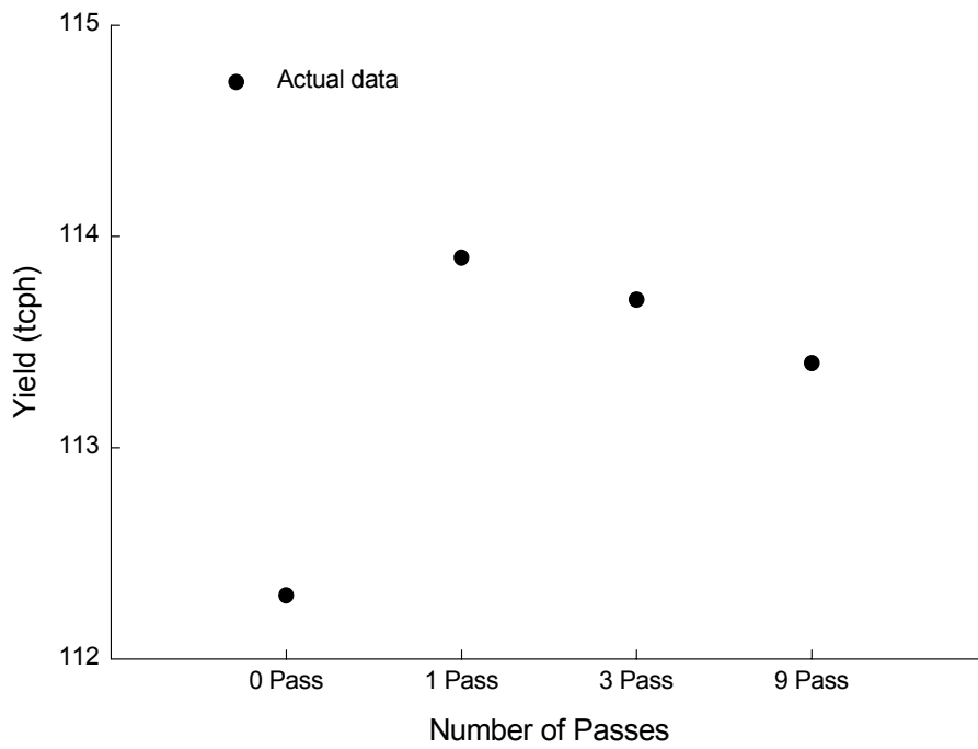
Figure 3: Yield of sugarcane after a varying number of tractor passes before planting
