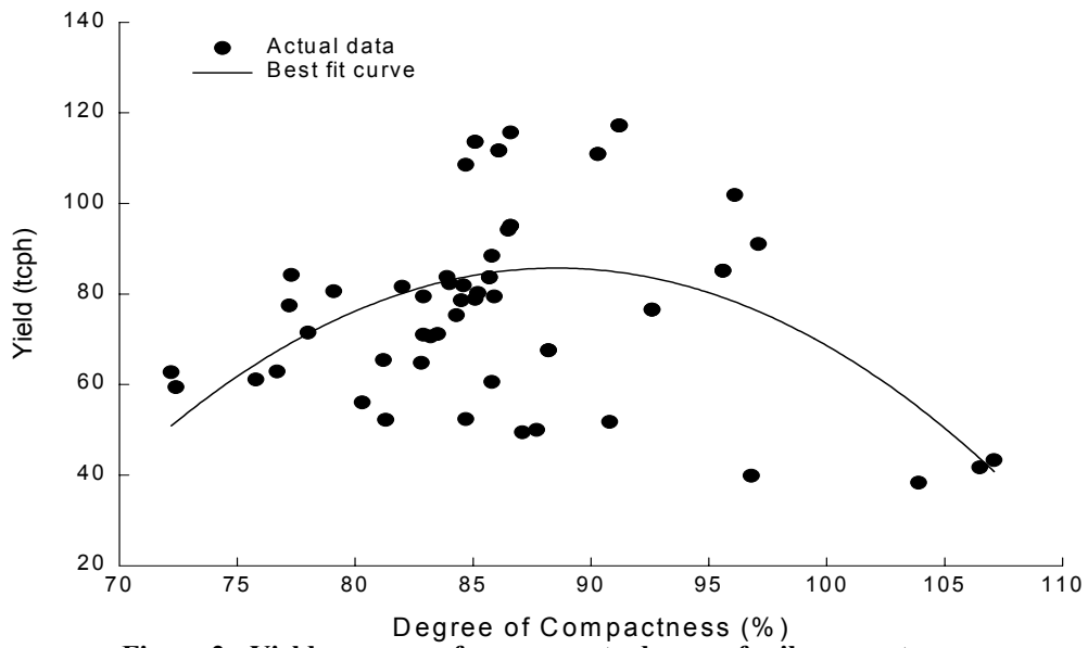
Figure 2: Yield response of sugarcane to degree of soil compactness
